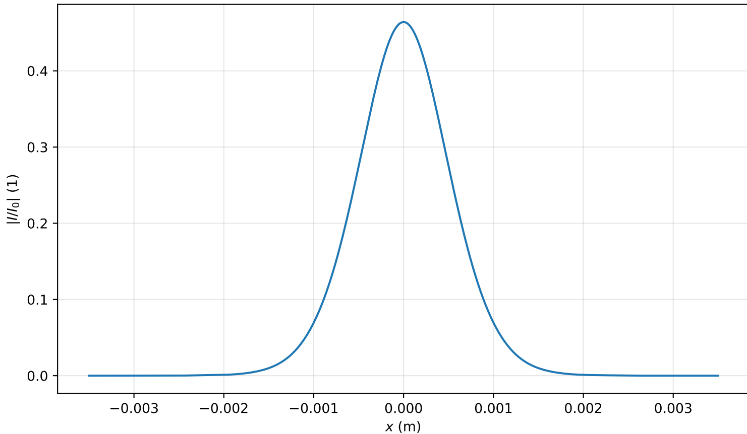
Intensity profile I(x, y = 0, z = 3.105m)/I_0 , P_{in}=0.4P_{cr} , artificial time
